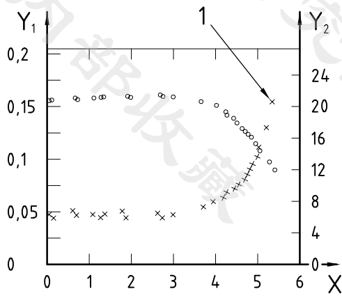
Figure B.1 — Typical hysteresis loop (Damping factor = 6,69 \times 10^{-2} , E' = 17,45 \text{ GN} \cdot \text{m}^{-2} , number of cycles = 8 986)
